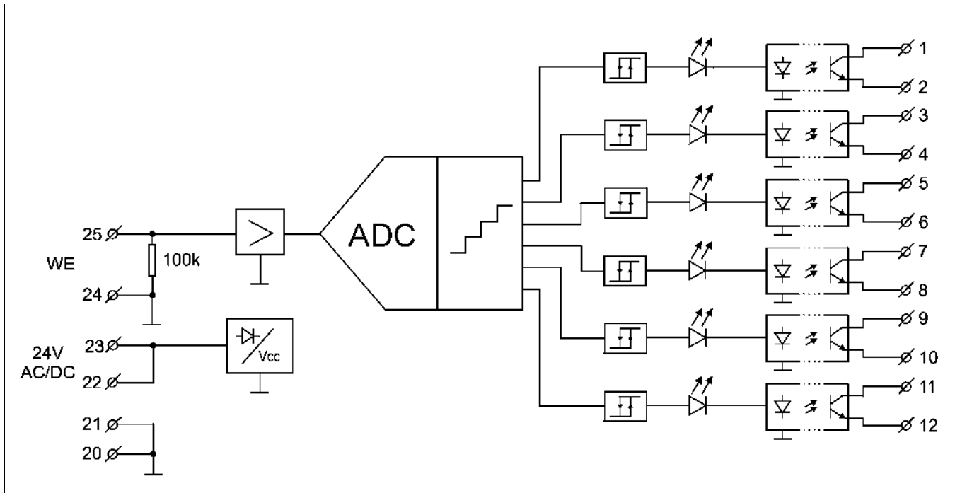
Fig.2 Connections of USS1360C.
