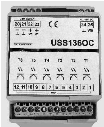
Fig.1 View of USS136OC.
