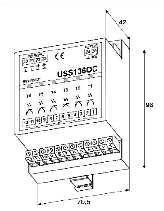
Fig.3 Dimensions of USS1360C.
