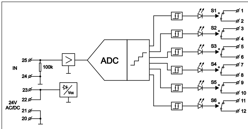
Fig.3 Connections of the URAC6NZ.
