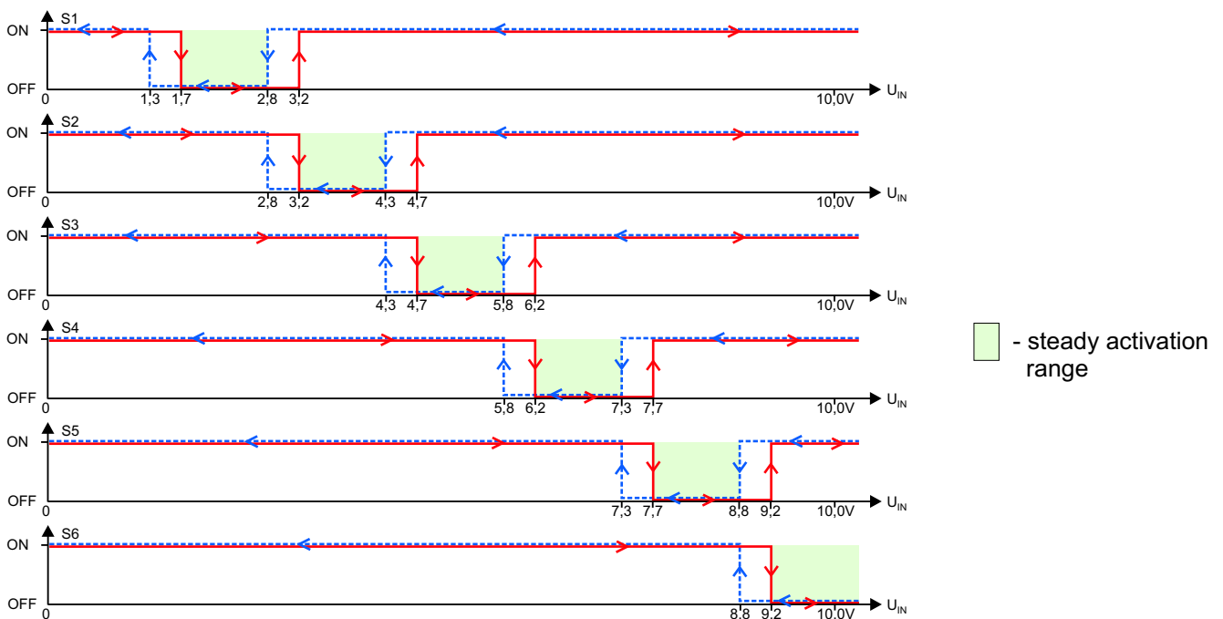
Fig.2 Switching diagram.
