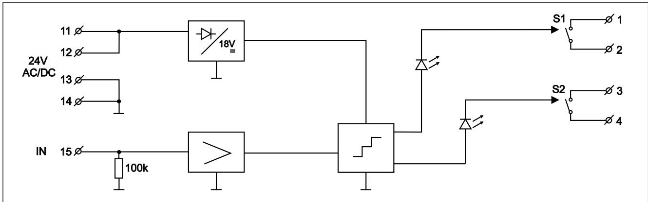
Fig.3 Connections of the USS121.
