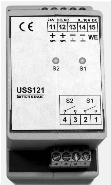
Fig.1 The USS121 module.
