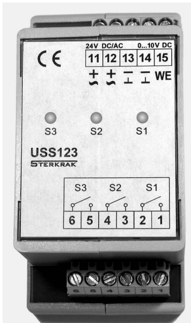
Fig.1 The USS123 module.
