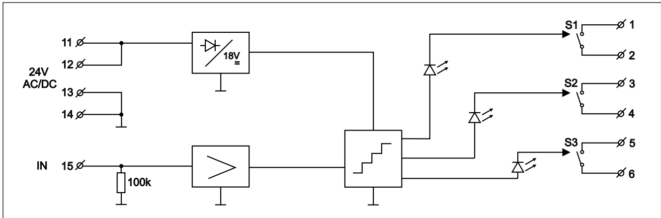
Fig.3 Connections of the USS123.
