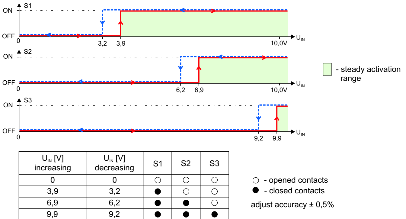
Fig.2 Switching diagram.
