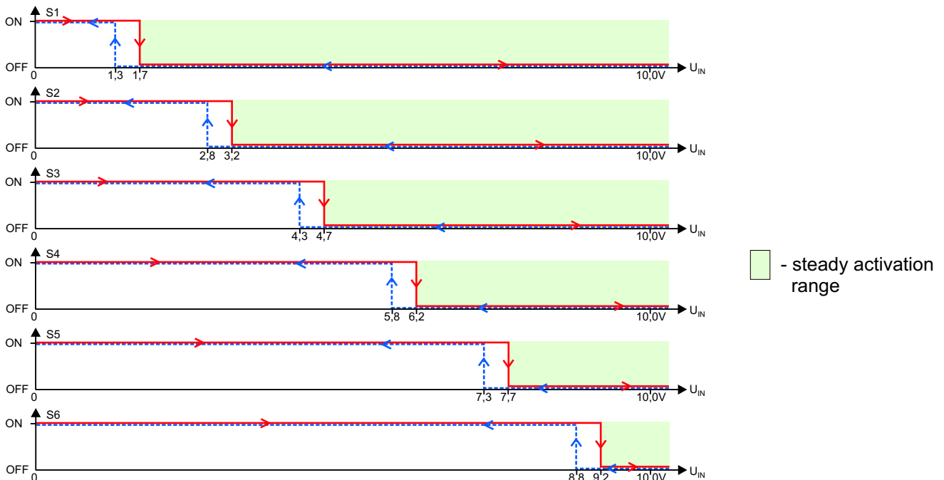
Fig.2 Switching diagram.
