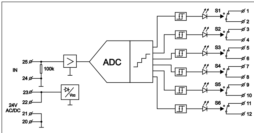
Fig.3 Connections of the USS136NZ.
