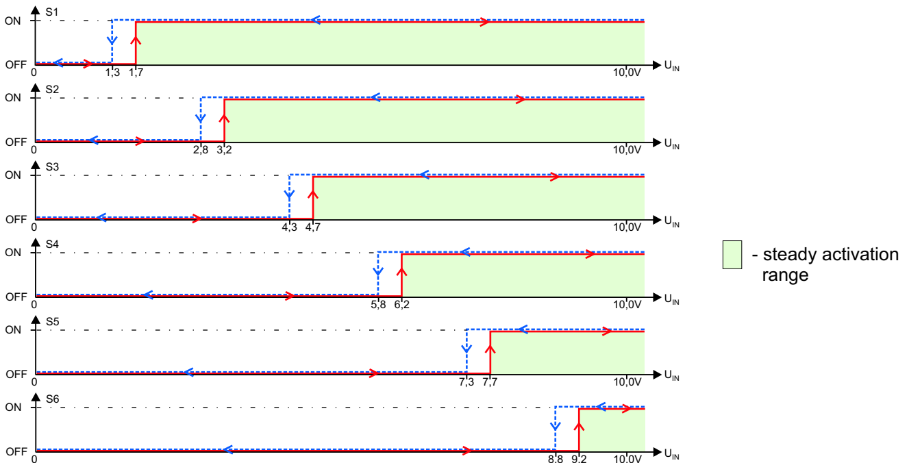
Fig.2 Switching diagram.
