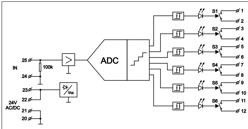
Fig.3 Connections of the USS136.
